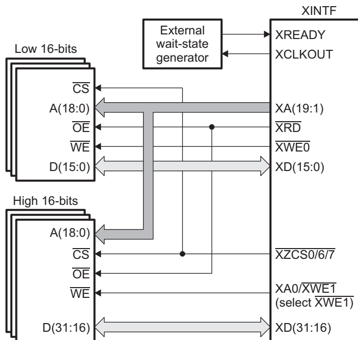
Figure 1-2. Typical 32-bit Data Bus XINTF Connections
