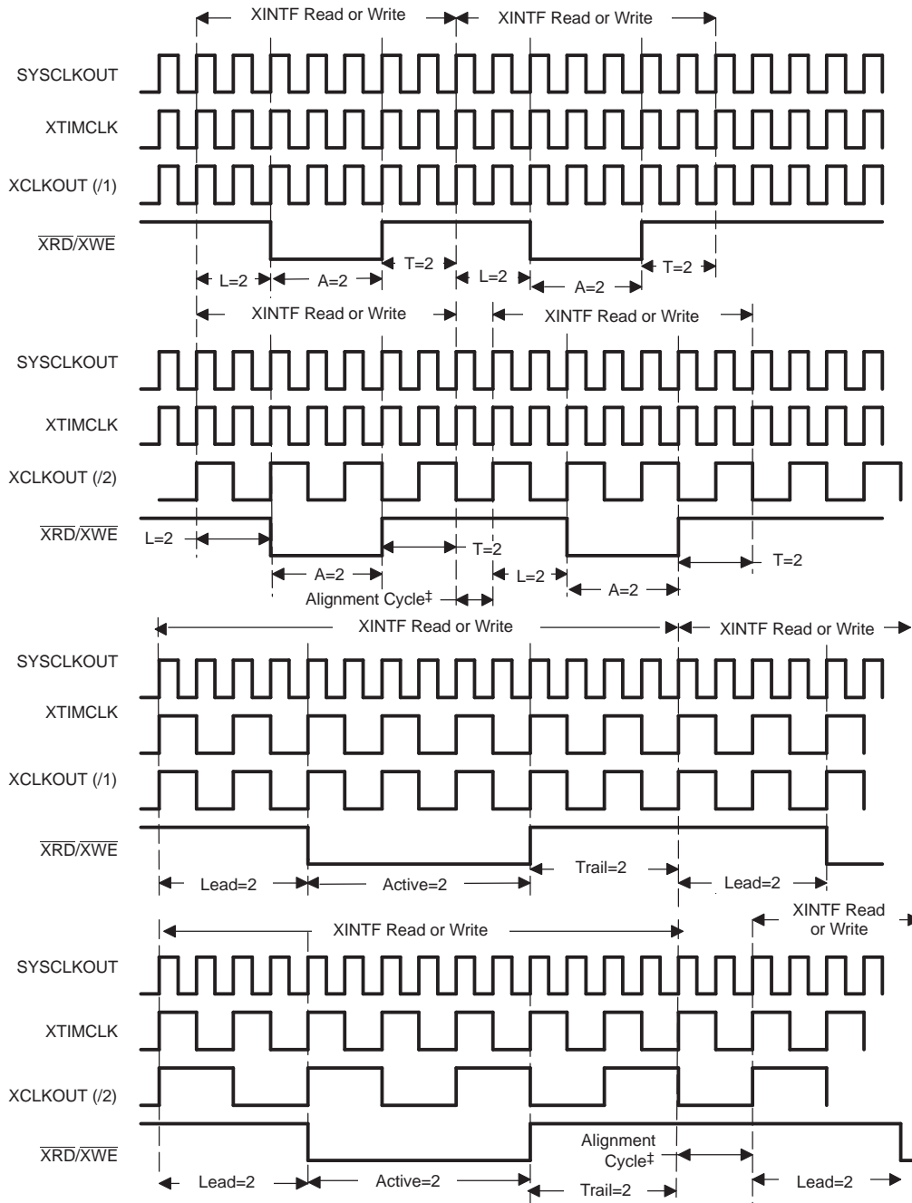
Figure 1-8. XTIMCLK and XCLKOUT Mode Waveforms
