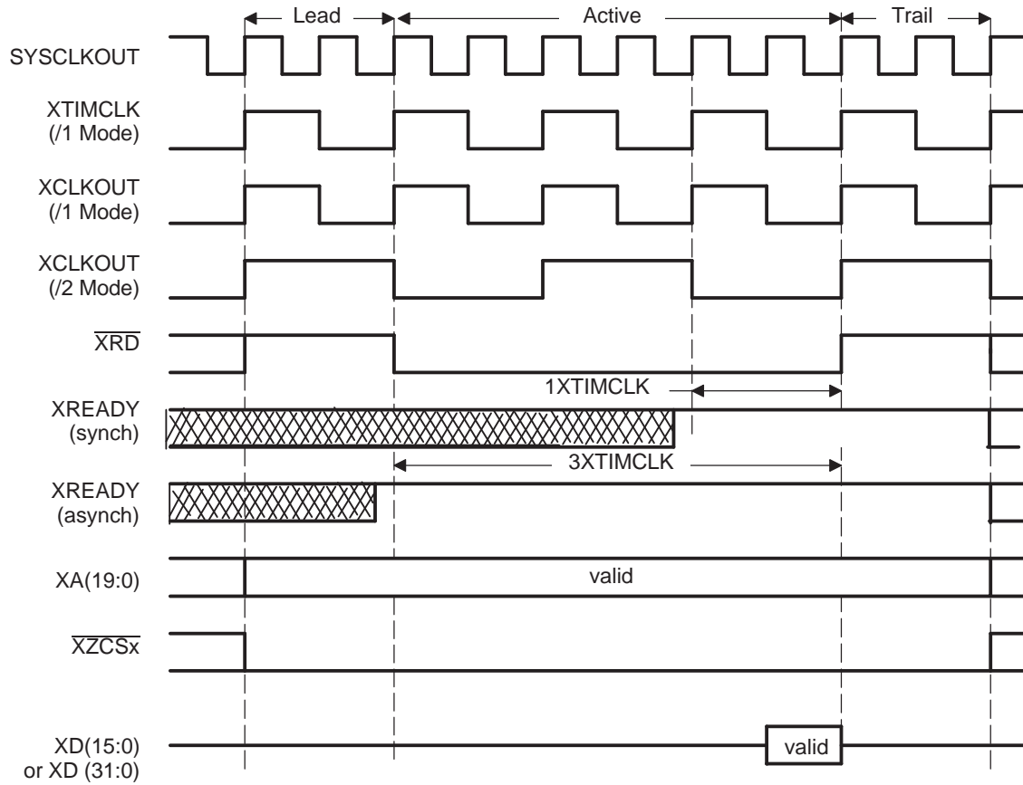
Figure 1-10. Generic Read Cycle (XTIMCLK = SYSCLKOUT mode)
