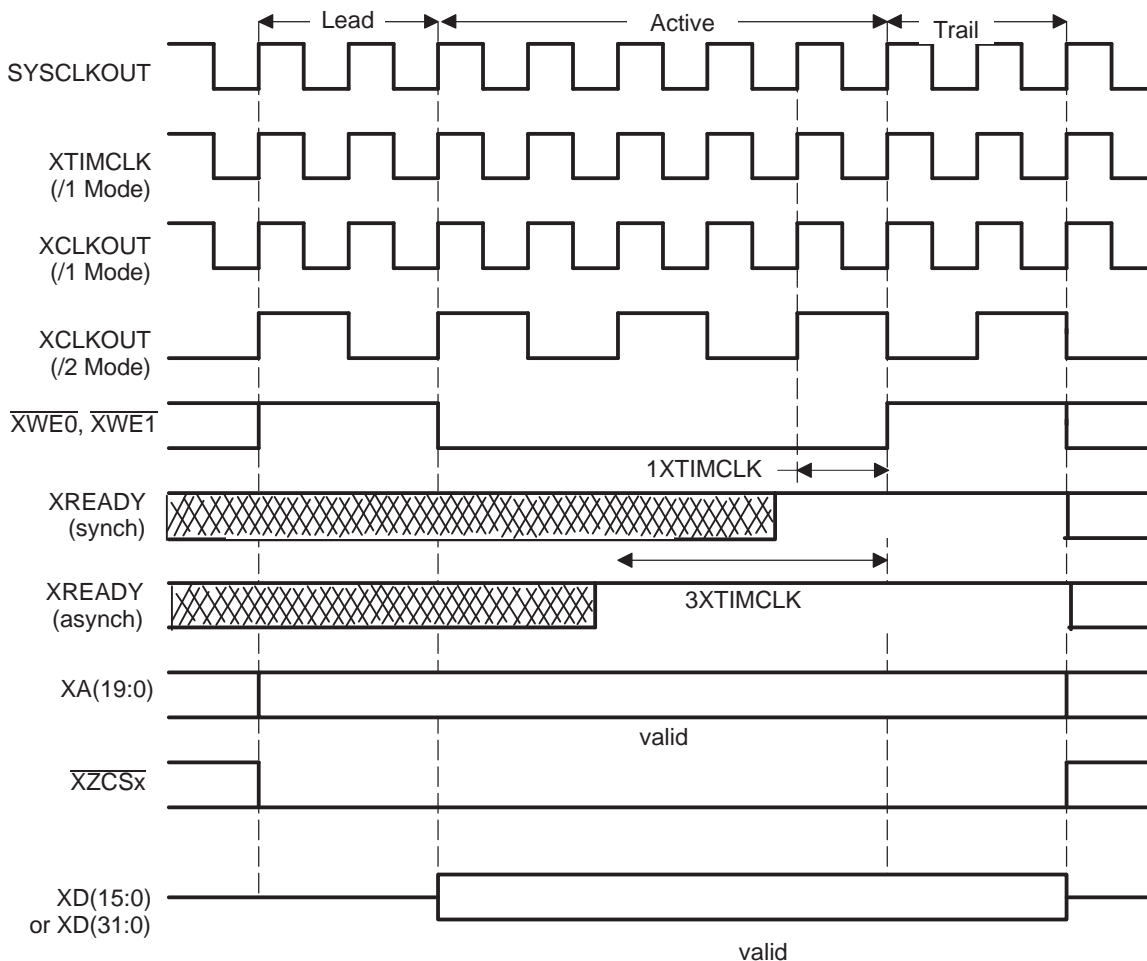
Figure 1-11. Generic Write Cycle (XTIMCLK = SYSCLKOUT mode)
