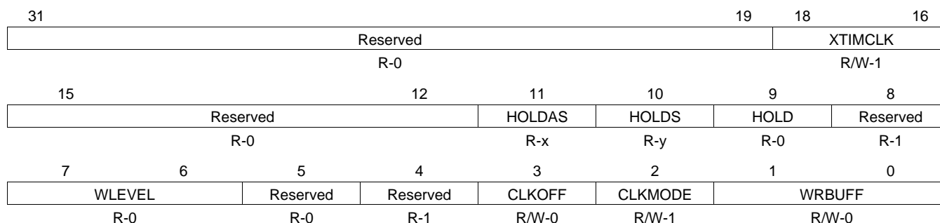
Figure 1-4. XINTF Configuration Register (XINTCNF2)
