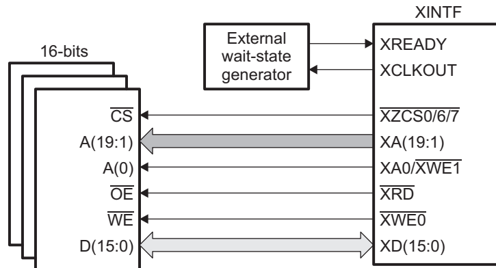
Figure 1-1. Typical 16-bit Data Bus XINTF Connections
